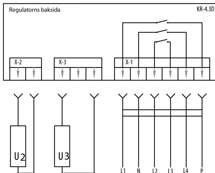
Fig. 12 Regulatorns kopplingschema
